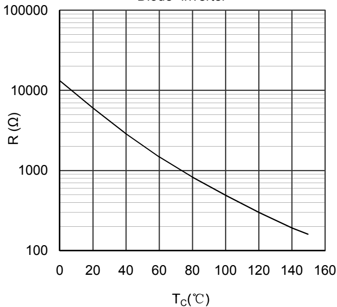
Figure 13. NTC Characteristics
