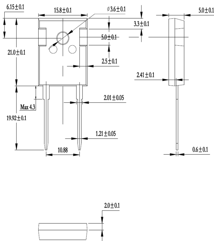
Figure 8. Package Outline
