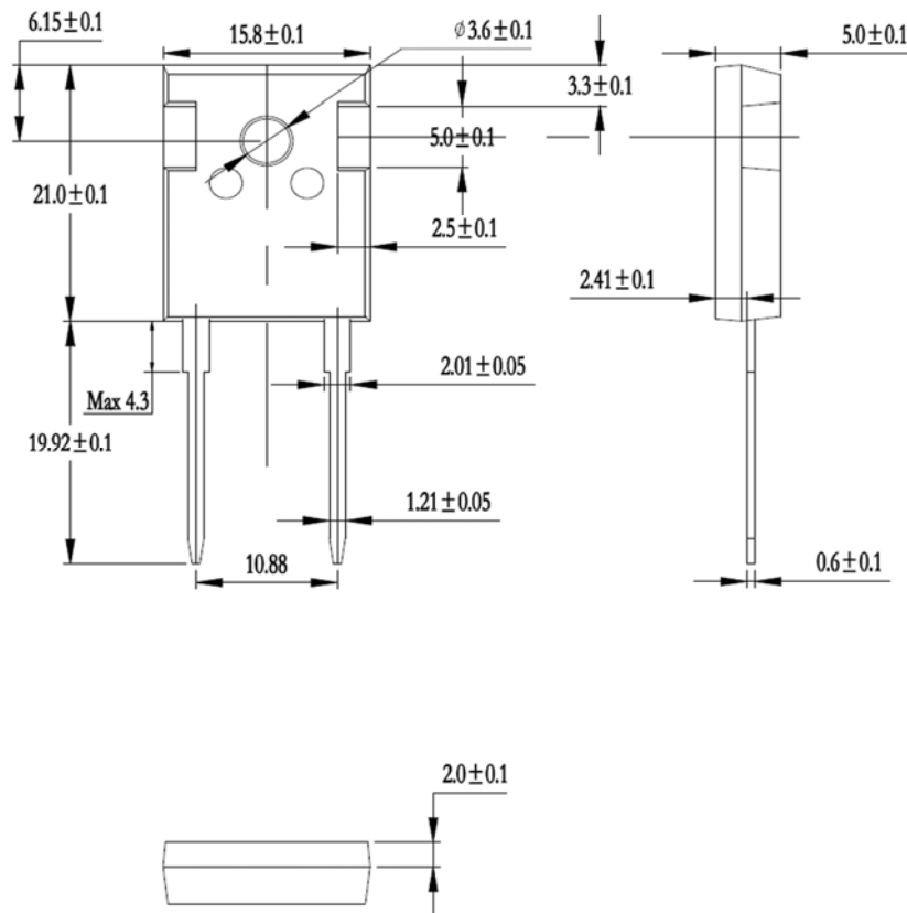
Dimensions in (mm) Figure 8. Package Outline
