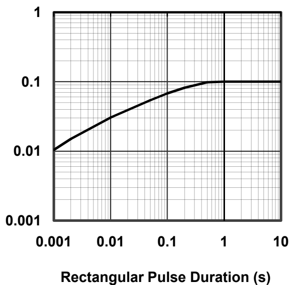
Figure 6. Transient Thermal Impedance
